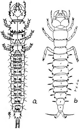
Fig. 22. Larvae: a, ground beetle, Pterostichus sp.; b, Dobsonfly, Corydalus cornutus (L.)
